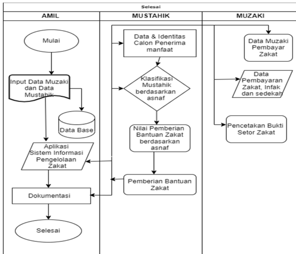
Gambar 3. Flowmap
