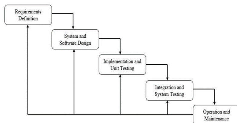
Gambar 1 Waterfall
